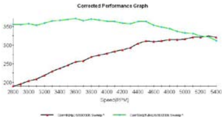
Dyno graph
